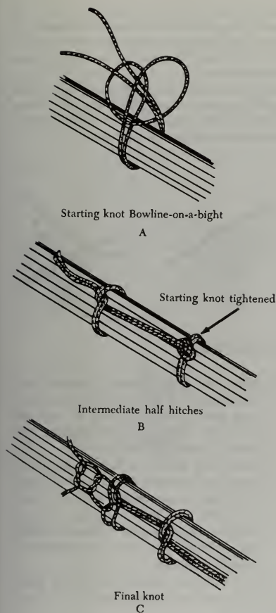
FIGURE 4-101. Double-cord lacing.
